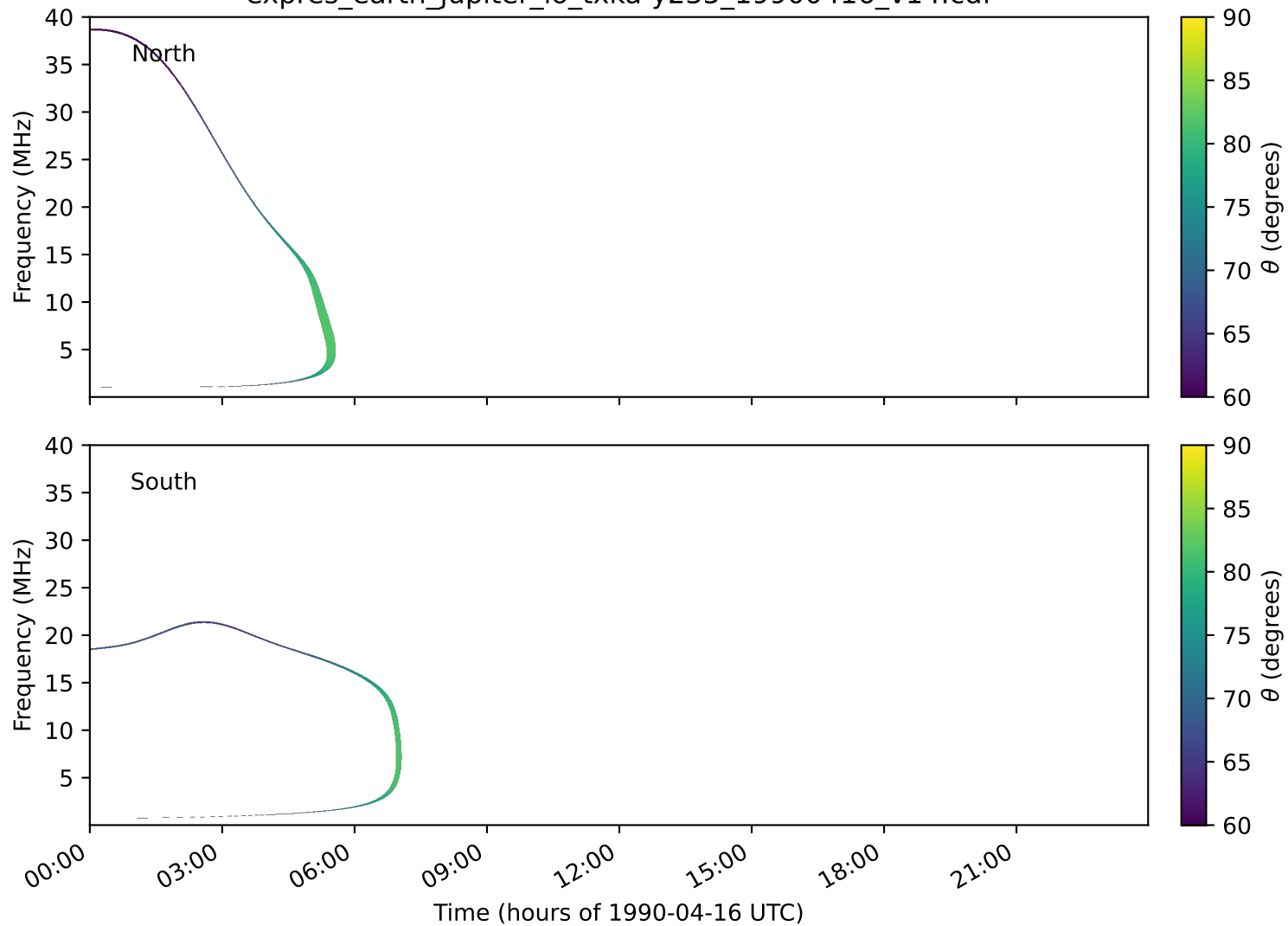
expres_earth_jupiter_io_txka-y235_19900416_v14.cdf
