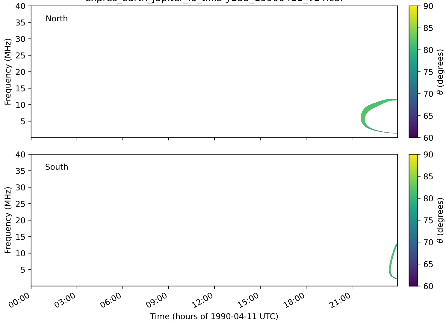
expres_earth_jupiter_io_txka-y235_19900411_v14.cdf
