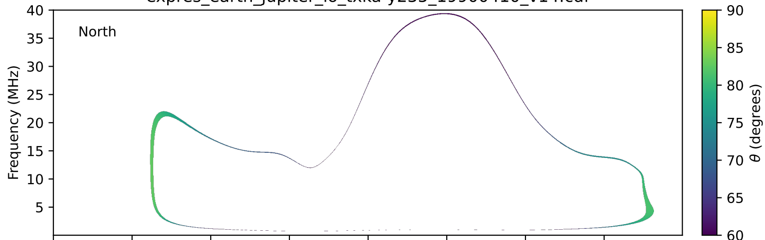
expres_earth_jupiter_io_txka-y235_19900410_v14.cdf
