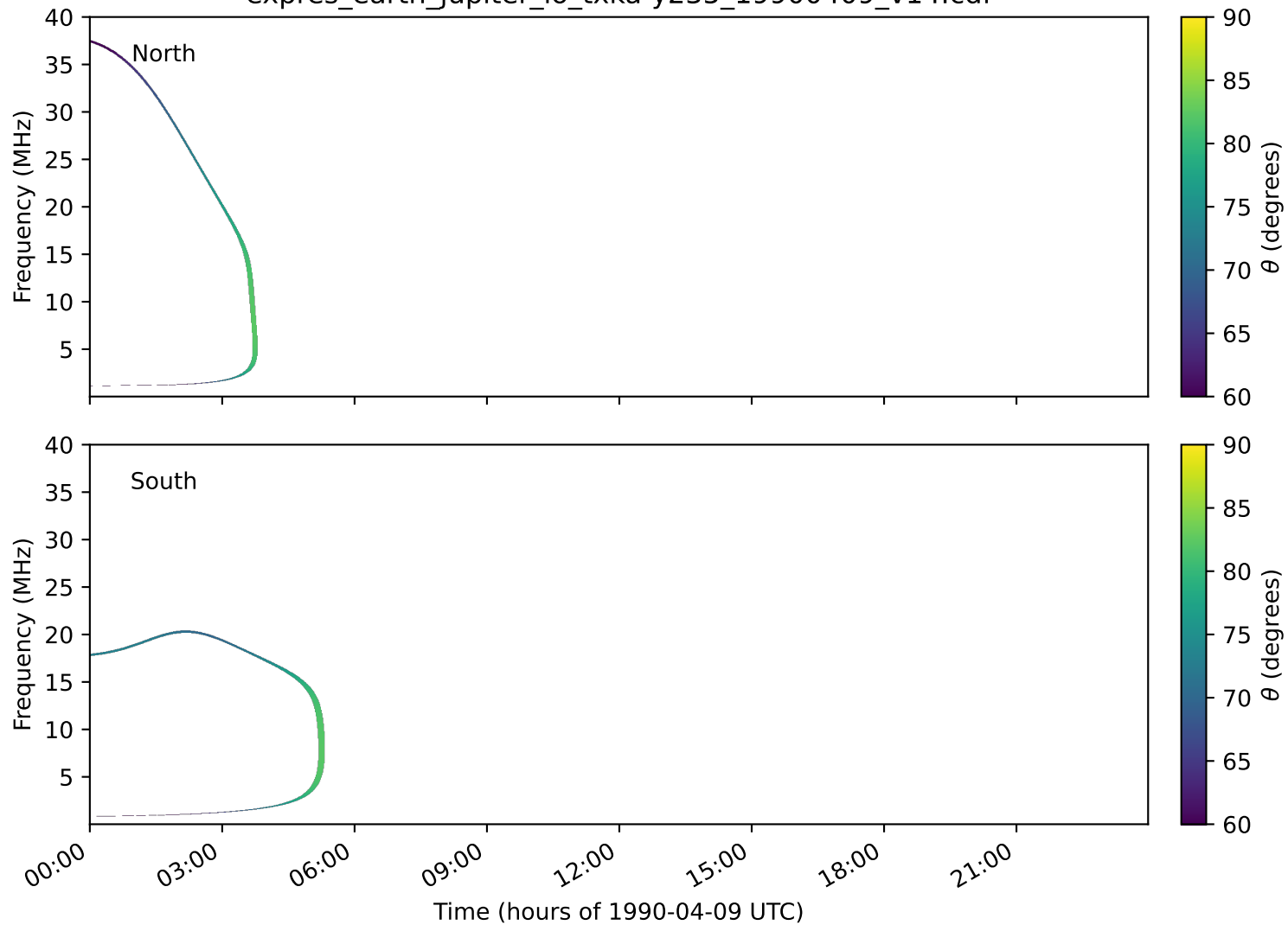
expres_earth_jupiter_io_txka-y235_19900409_v14.cdf
