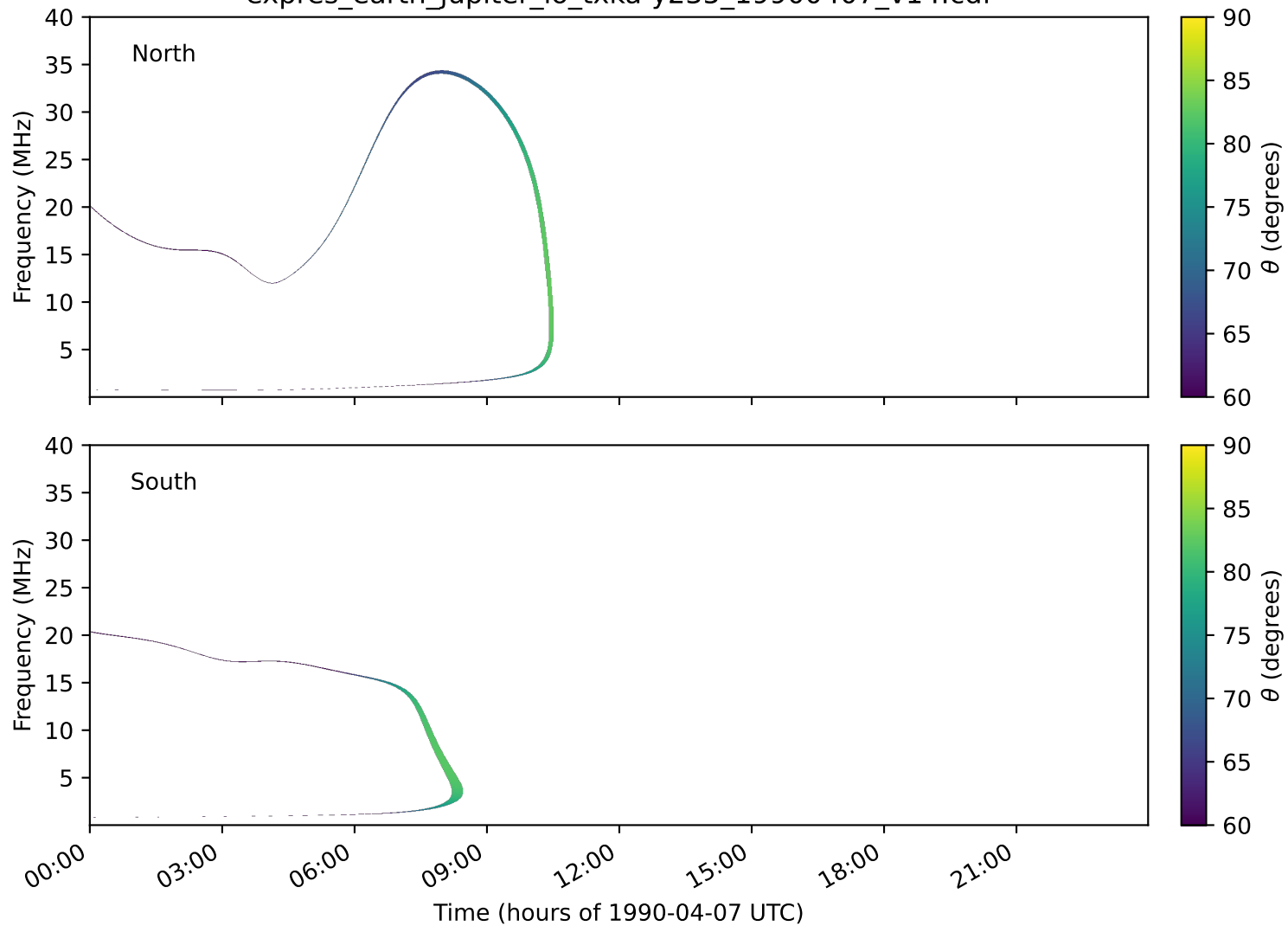
expres_earth_jupiter_io_txka-y235_19900407_v14.cdf
