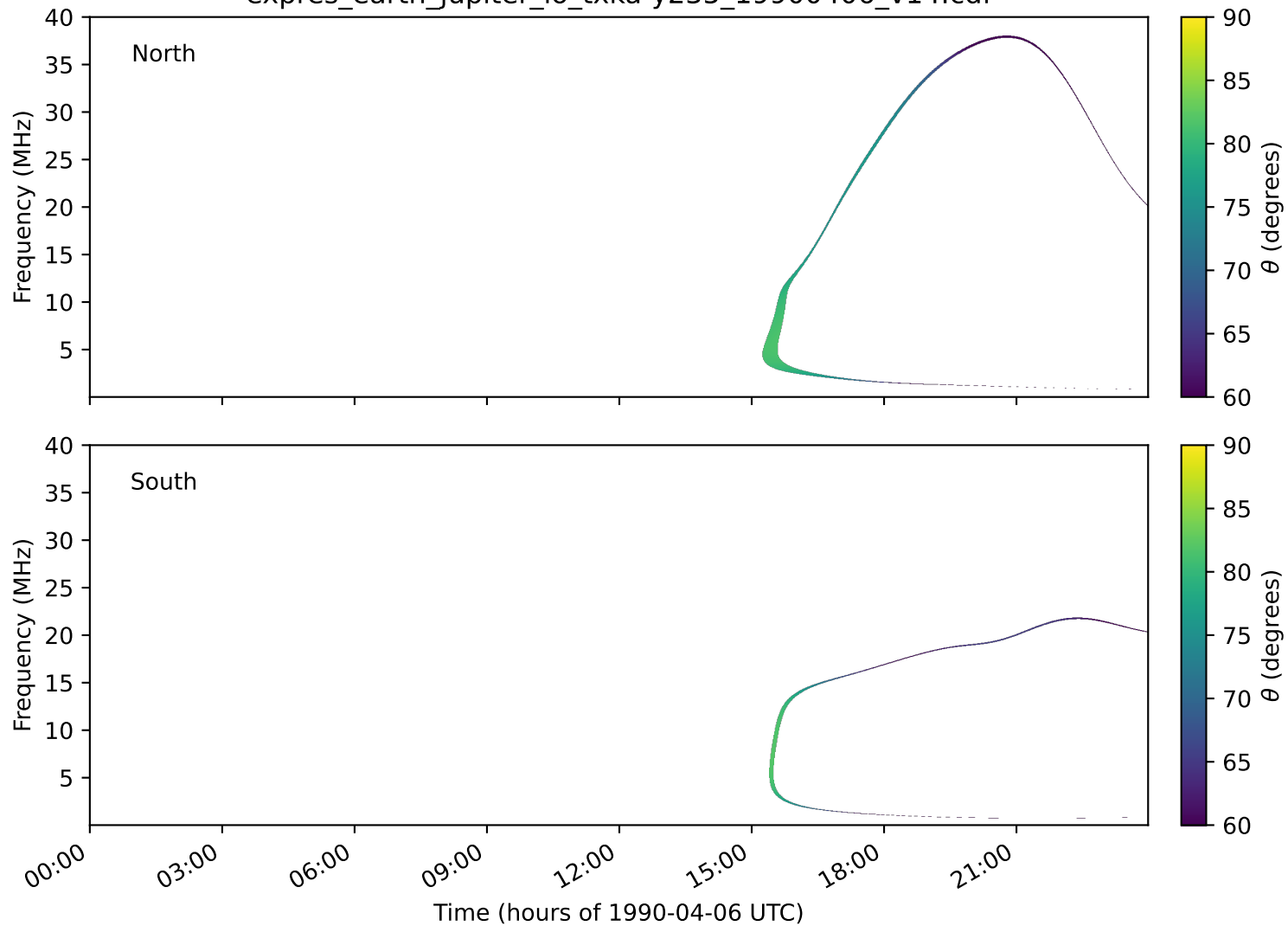
expres_earth_jupiter_io_txka-y235_19900406_v14.cdf
