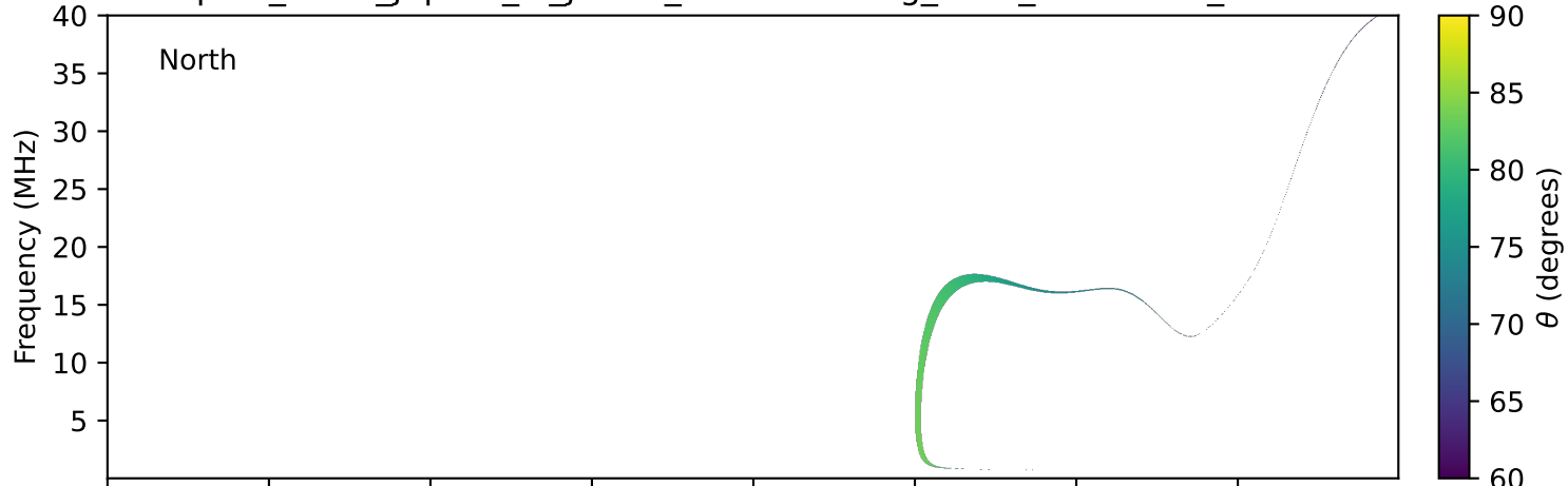
expres_earth_jupiter_io_jrm33_lossc-wid1deg_3kev_19900429_v11.cdf
