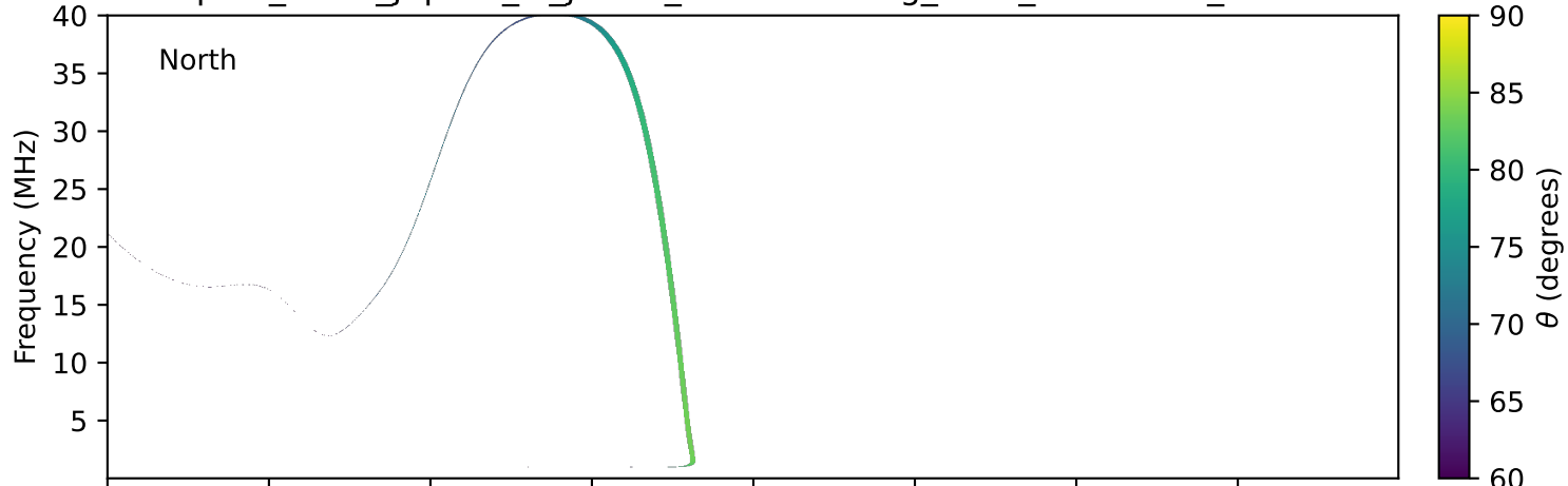
expres_earth_jupiter_io_jrm33_lossc-wid1deg_3kev_19900407_v11.cdf
