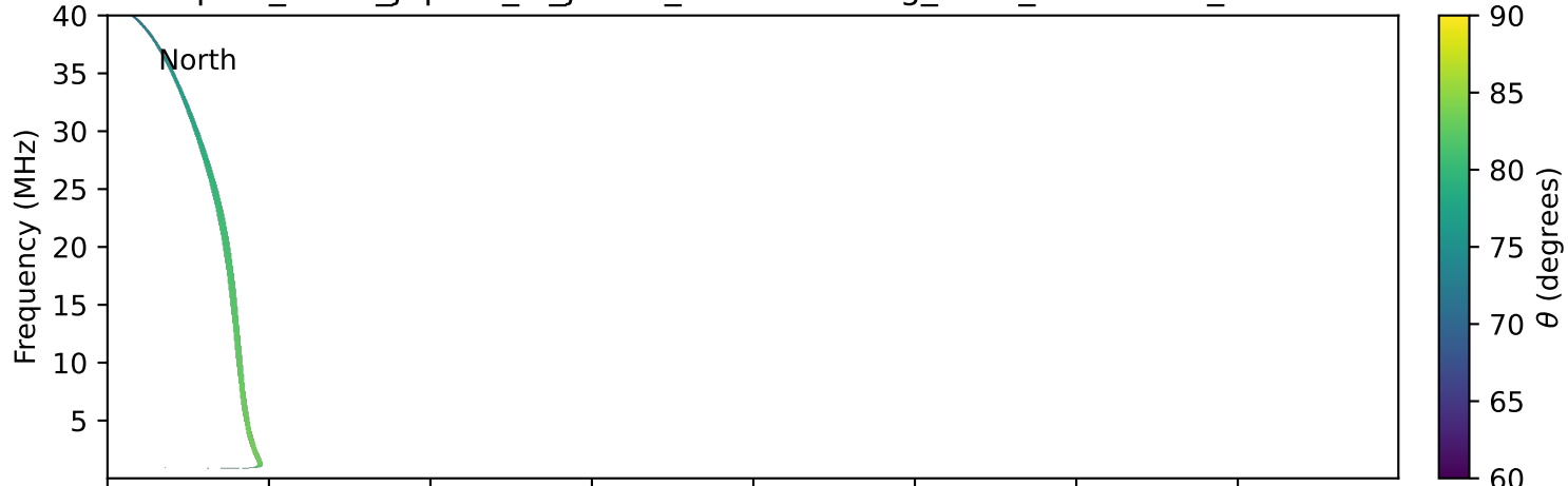
expres_earth_jupiter_io_jrm33_lossc-wid1deg_3kev_19900402_v11.cdf
