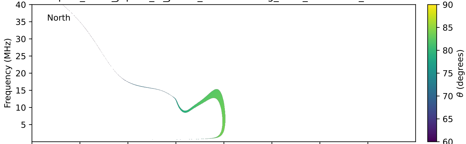
expres_earth_jupiter_io_jrm09_lossc-wid1deg_3kev_19900430_v11.cdf
