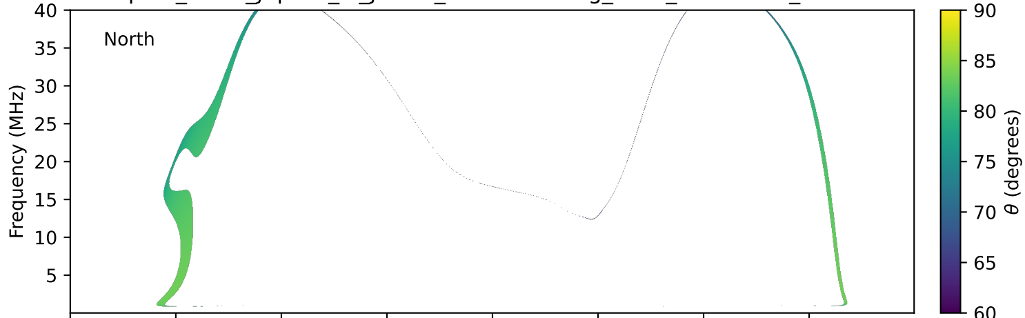
expres_earth_jupiter_io_jrm09_lossc-wid1deg_3kev_19900426_v11.cdf
