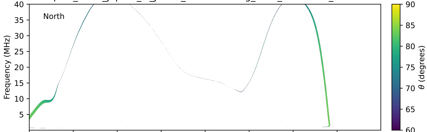
expres_earth_jupiter_io_jrm09_lossc-wid1deg_3kev_19900419_v11.cdf
