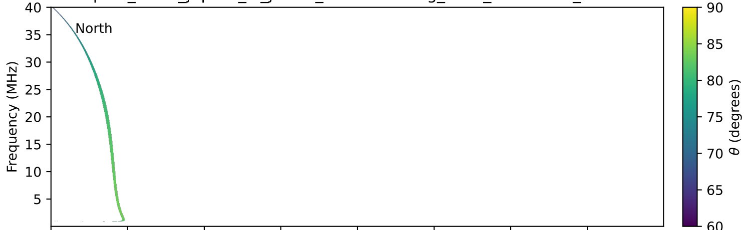
expres_earth_jupiter_io_jrm09_lossc-wid1deg_3kev_19900402_v11.cdf
