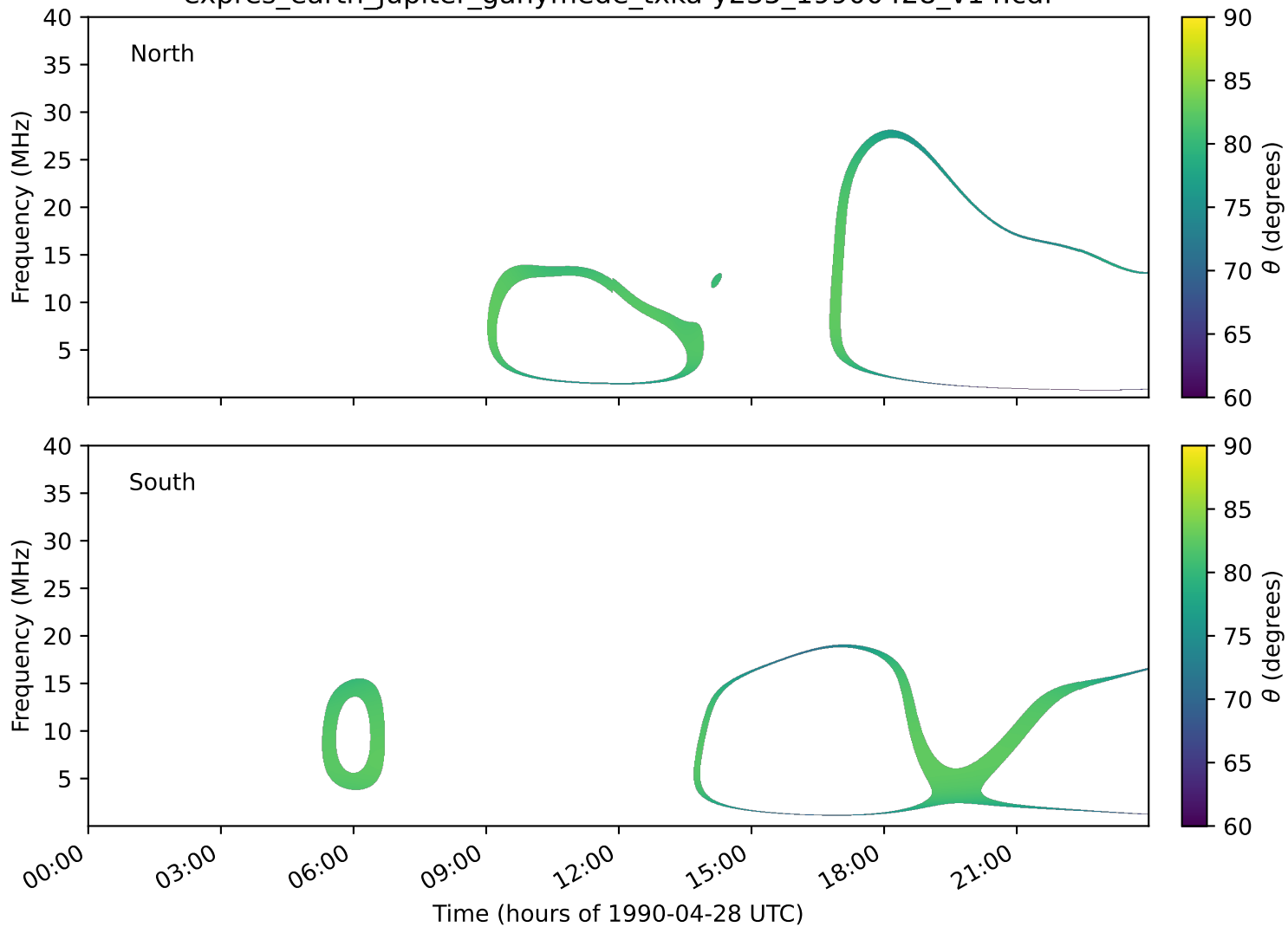
expres_earth_jupiter_ganymede_txka-y235_19900428_v14.cdf
