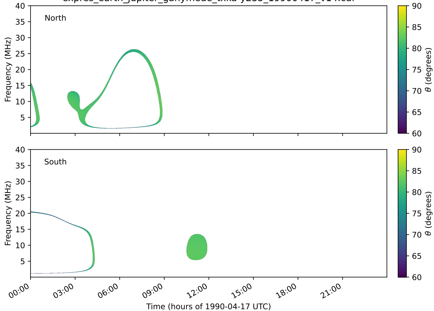
expres_earth_jupiter_ganymede_txka-y235_19900417_v14.cdf
