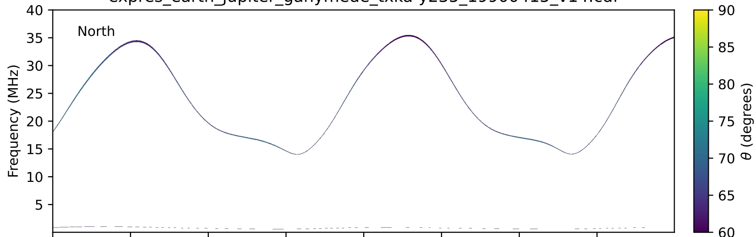
expres_earth_jupiter_ganymede_txka-y235_19900415_v14.cdf
