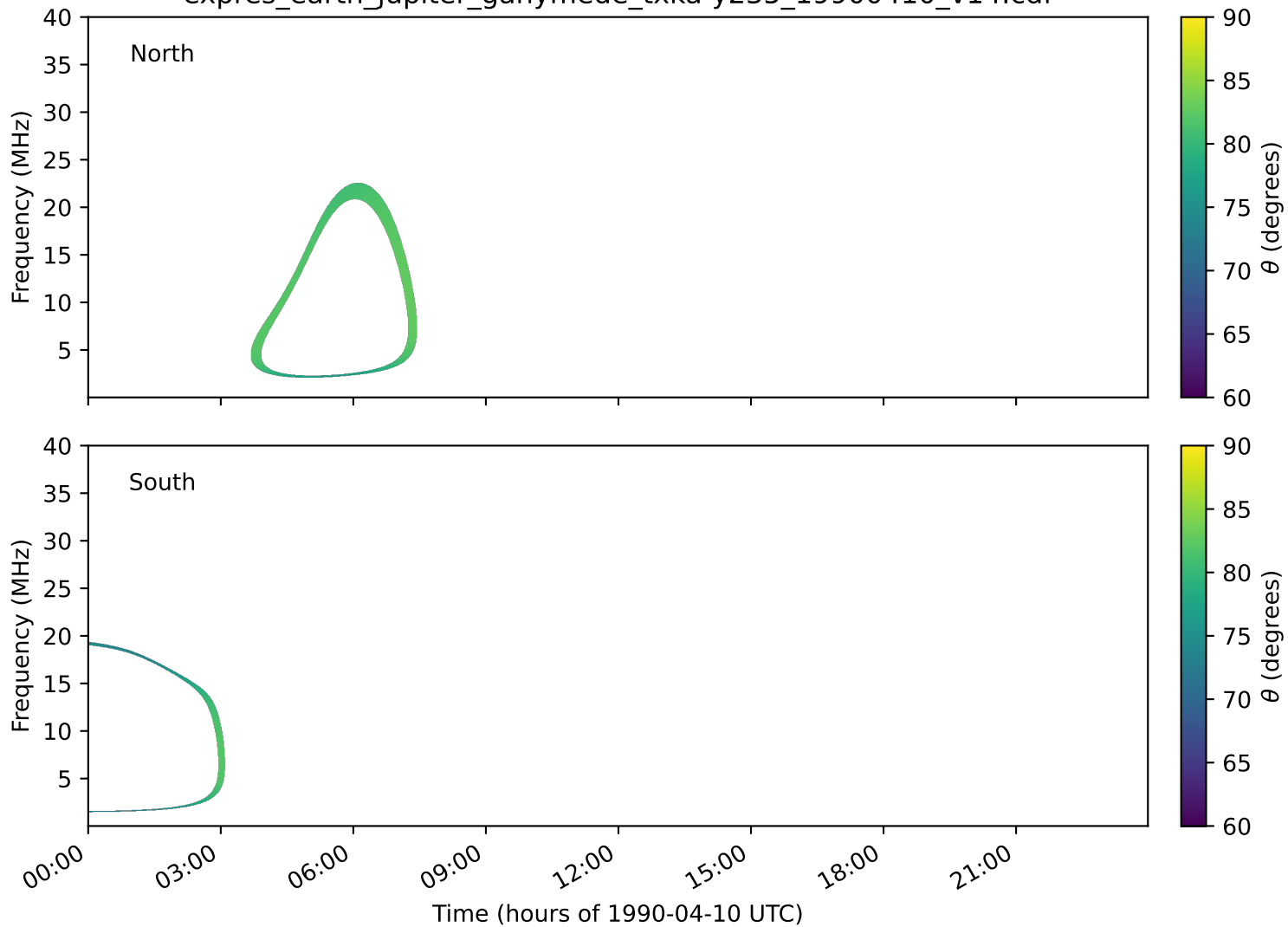
expres_earth_jupiter_ganymede_txka-y235_19900410_v14.cdf
