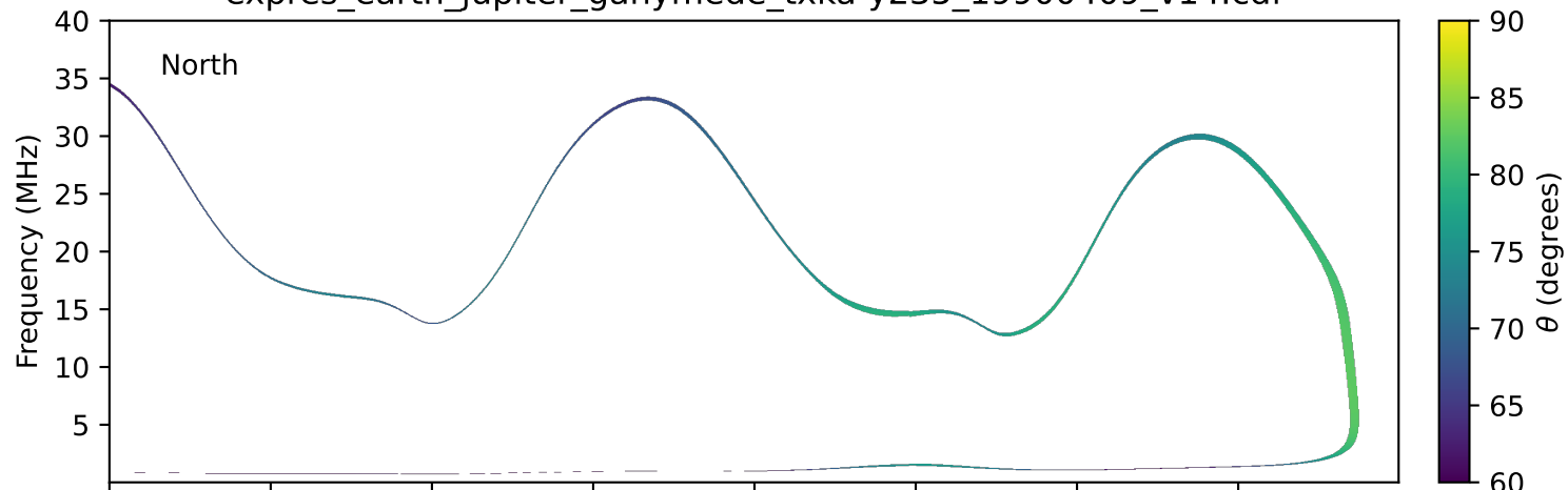
expres_earth_jupiter_ganymede_txka-y235_19900409_v14.cdf
