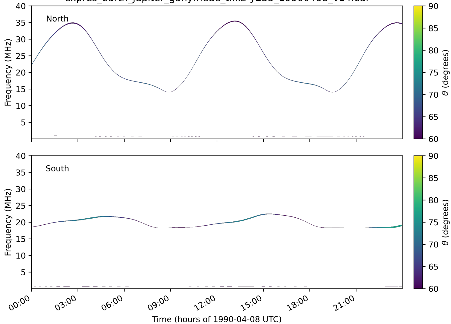
expres_earth_jupiter_ganymede_txka-y235_19900408_v14.cdf
