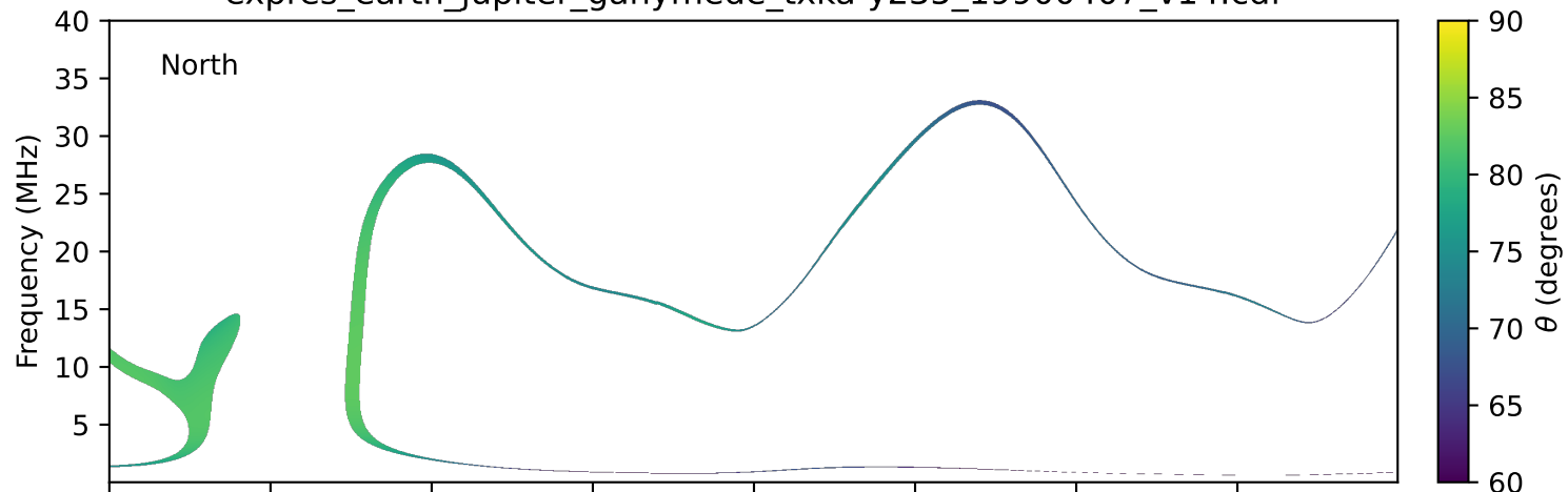
expres_earth_jupiter_ganymede_txka-y235_19900407_v14.cdf
