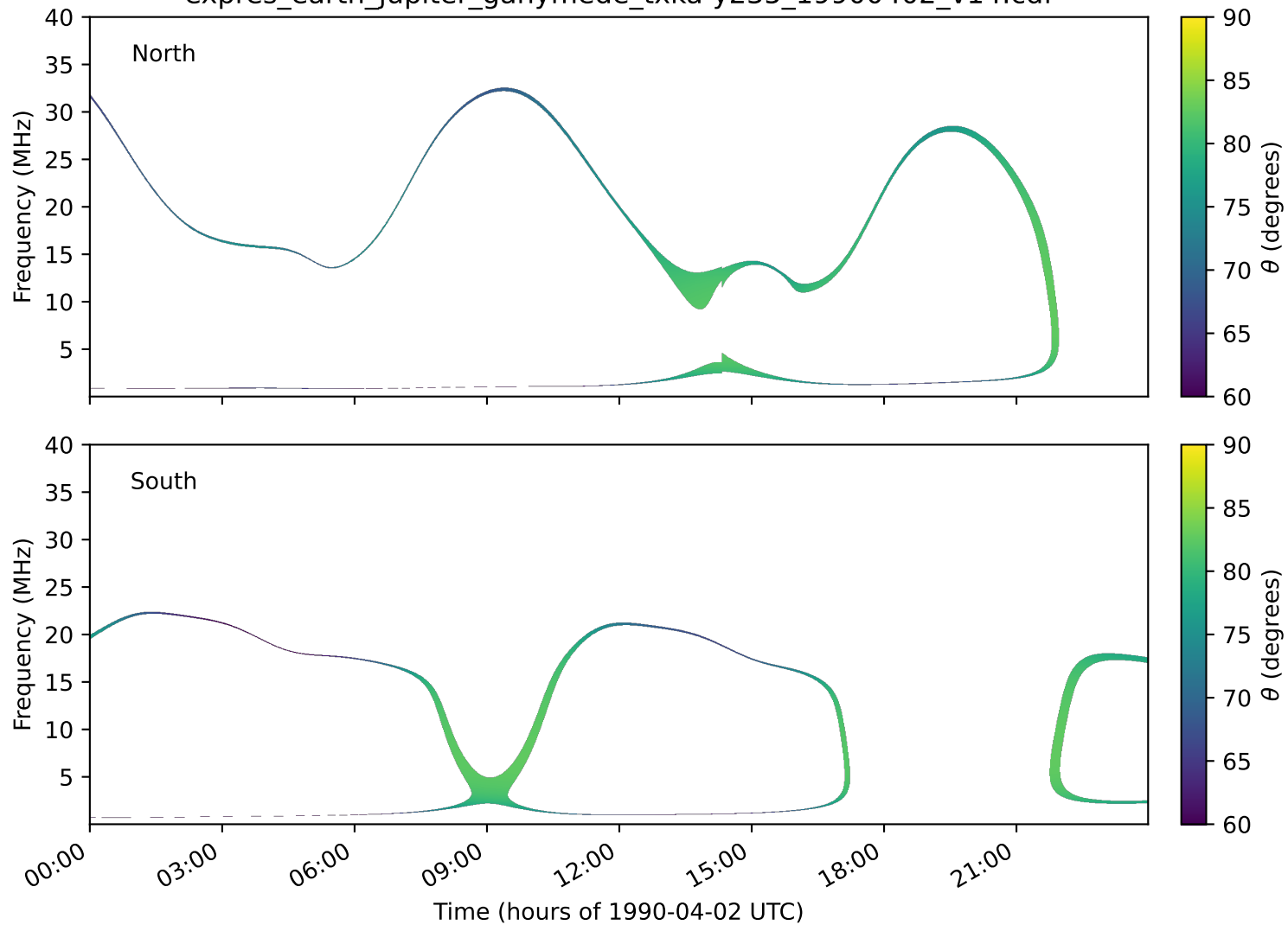
expres_earth_jupiter_ganymede_txka-y235_19900402_v14.cdf
