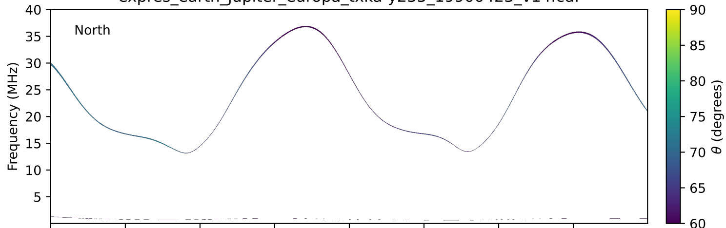
expres_earth_jupiter_europa_txka-y235_19900423_v14.cdf
