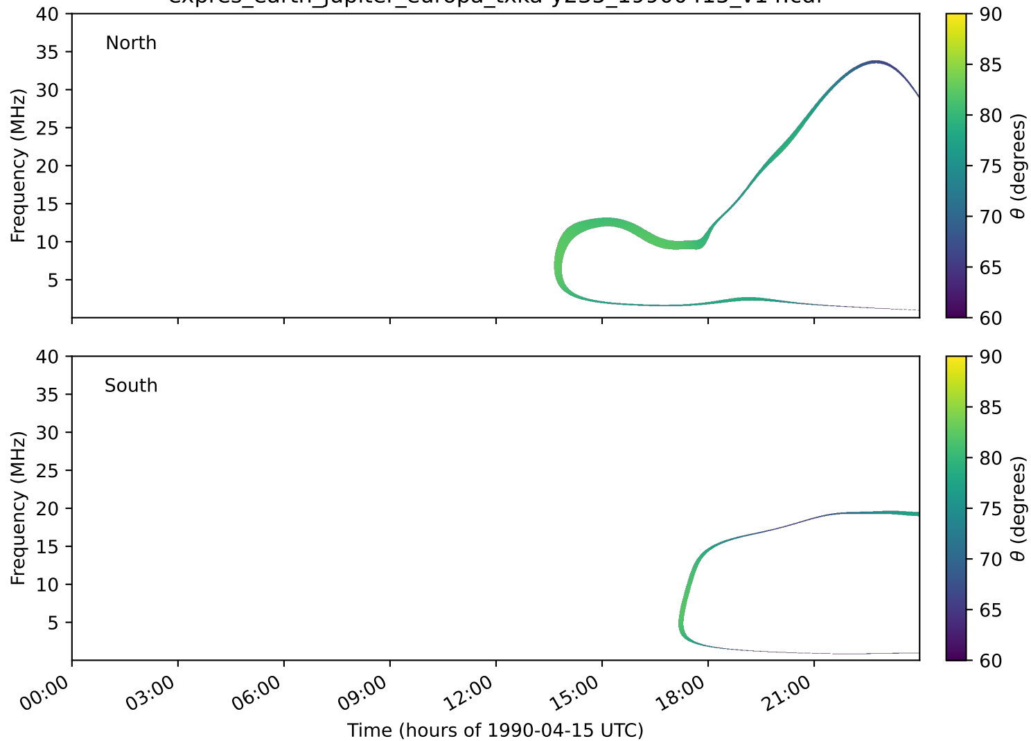
expres_earth_jupiter_europa_txka-y235_19900415_v14.cdf
