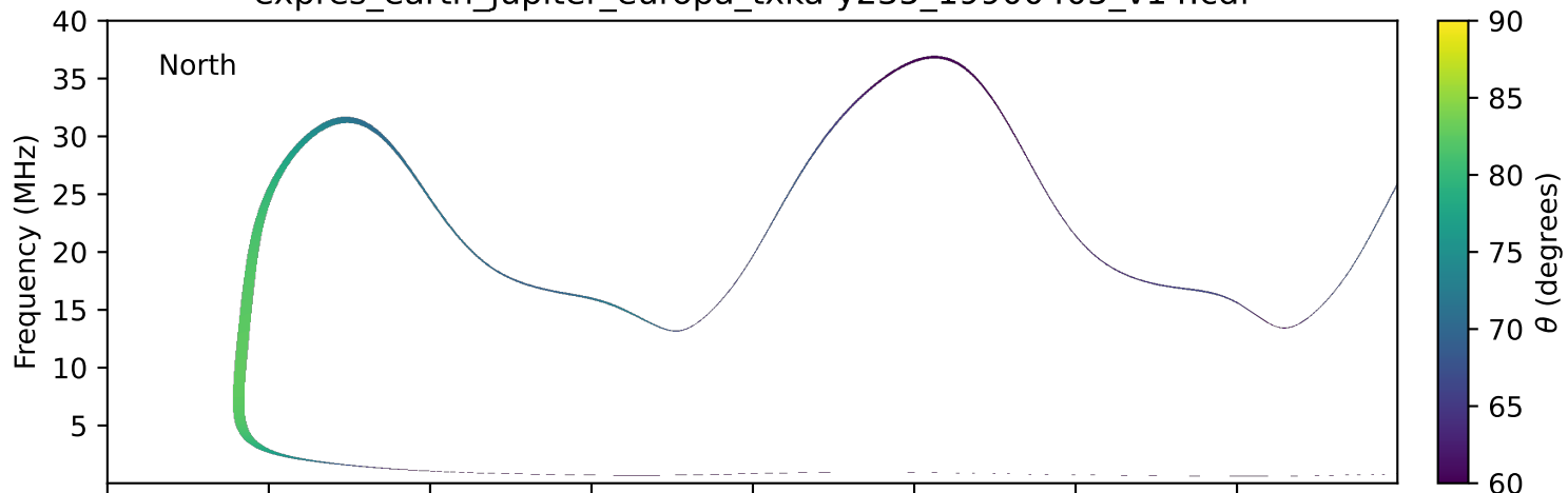
expres_earth_jupiter_europa_txka-y235_19900405_v14.cdf
