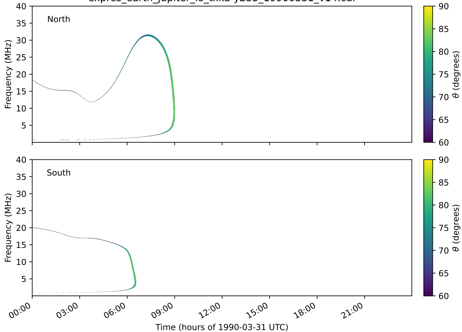
expres_earth_jupiter_io_txka-y235_19900331_v14.cdf
