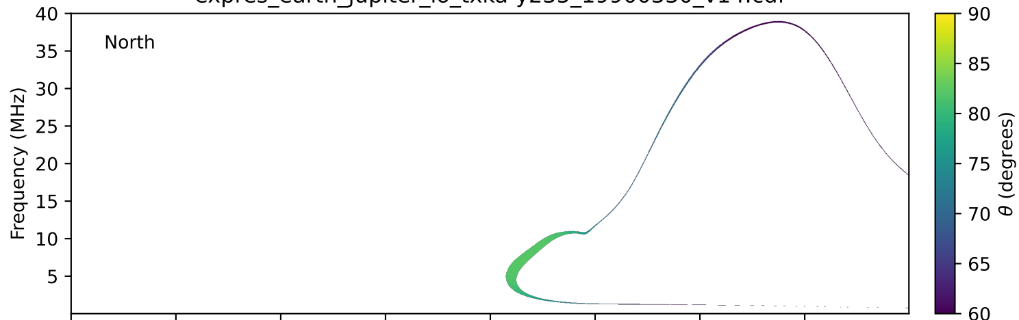
expres_earth_jupiter_io_txka-y235_19900330_v14.cdf
