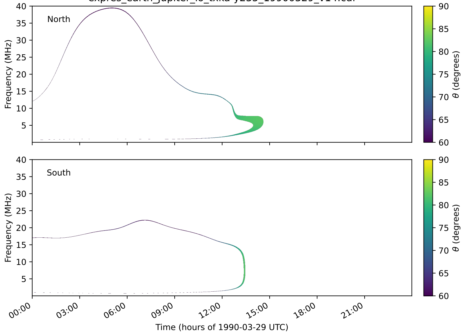
expres_earth_jupiter_io_txka-y235_19900329_v14.cdf
