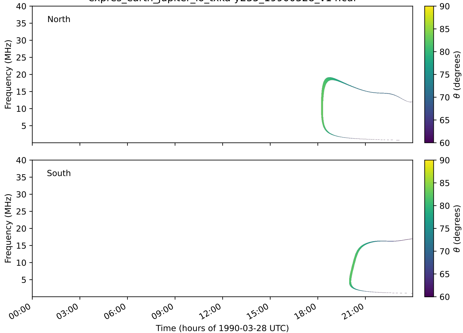
expres_earth_jupiter_io_txka-y235_19900328_v14.cdf
