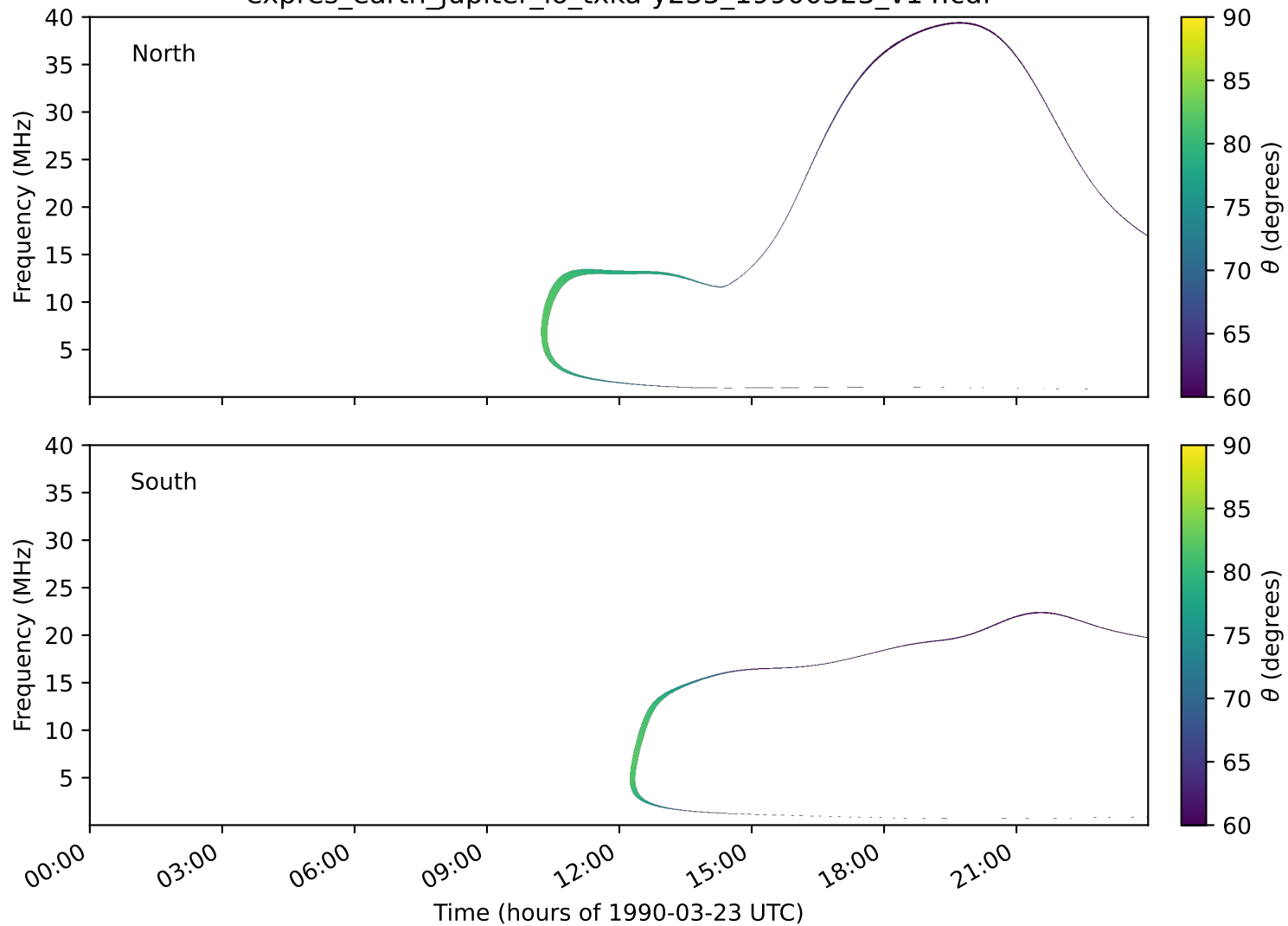
expres_earth_jupiter_io_txka-y235_19900323_v14.cdf
