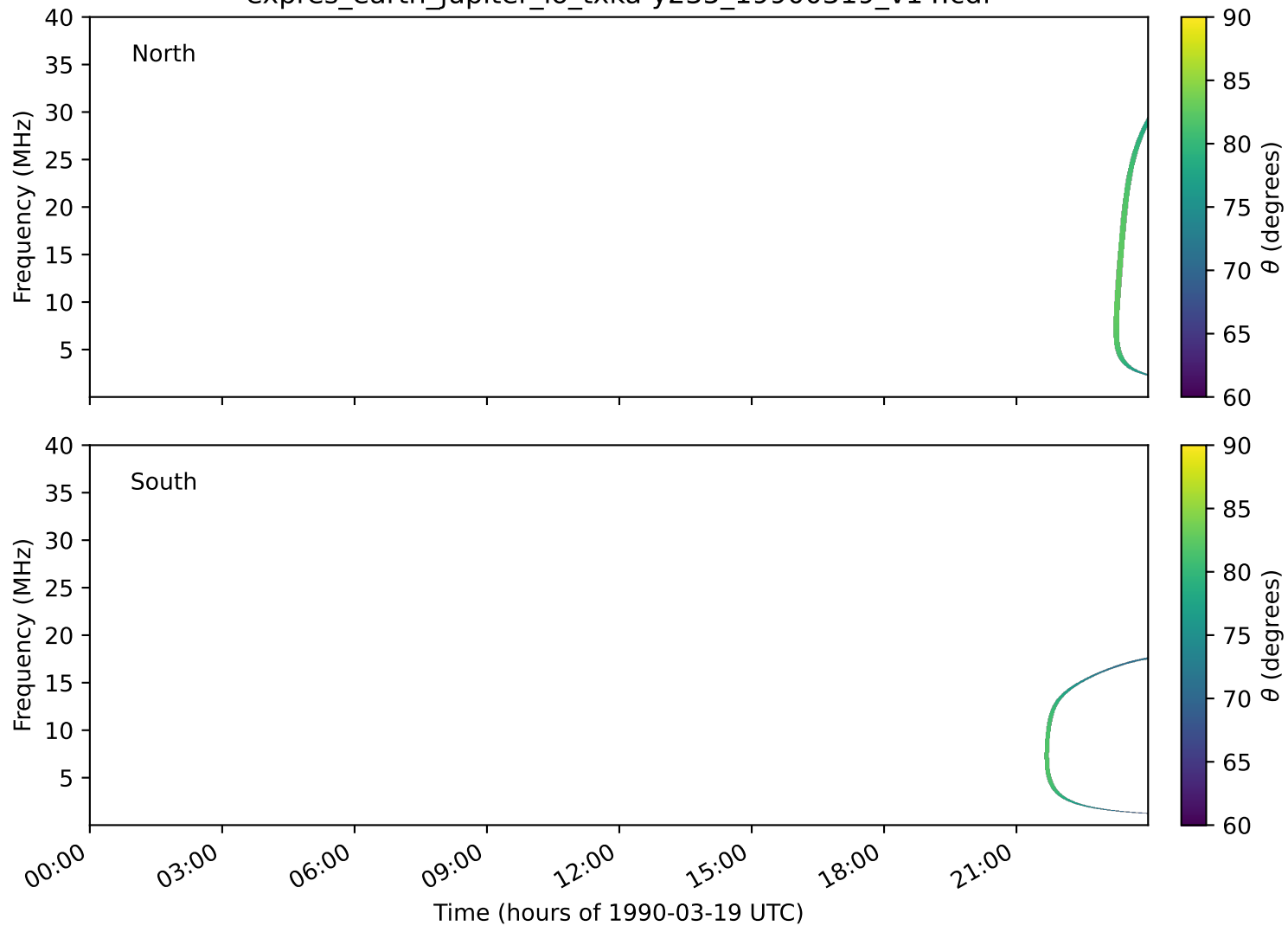
expres_earth_jupiter_io_txka-y235_19900319_v14.cdf
