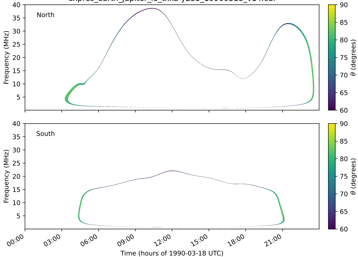
expres_earth_jupiter_io_txka-y235_19900318_v14.cdf
