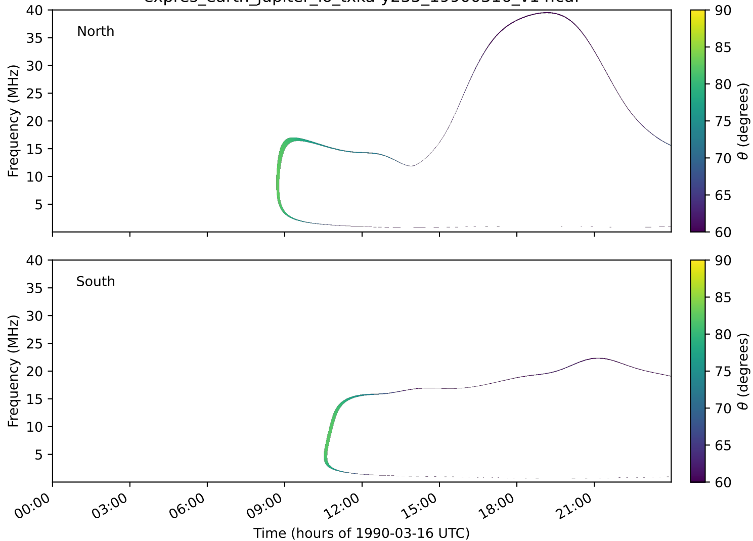
expres_earth_jupiter_io_txka-y235_19900316_v14.cdf
