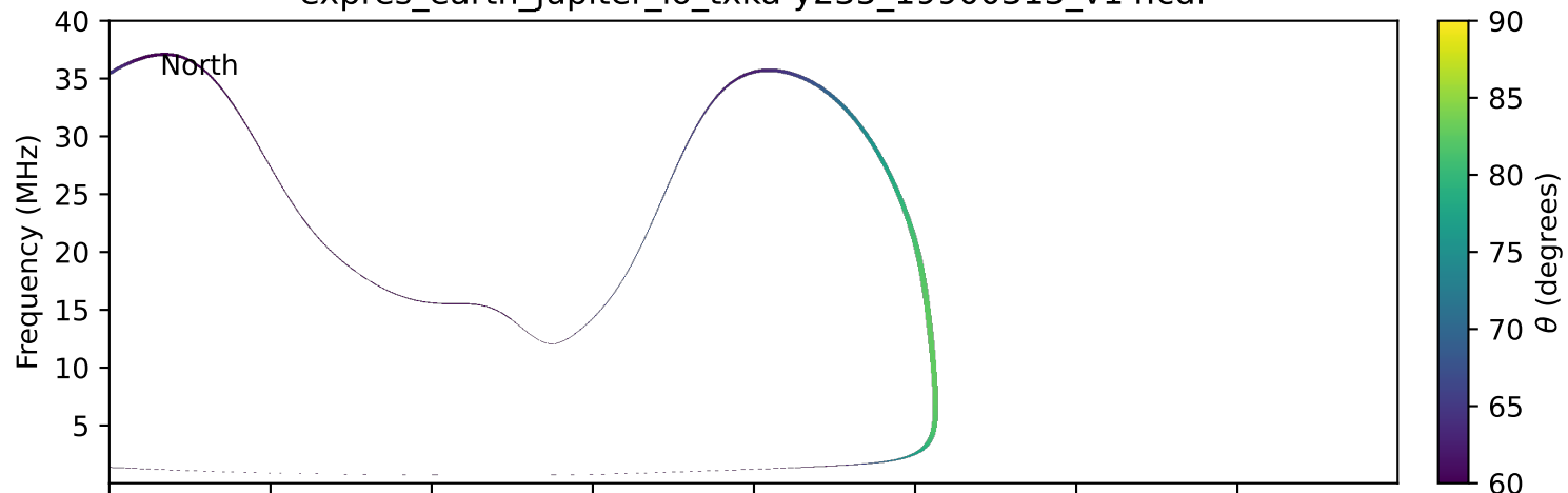
expres_earth_jupiter_io_txka-y235_19900313_v14.cdf
