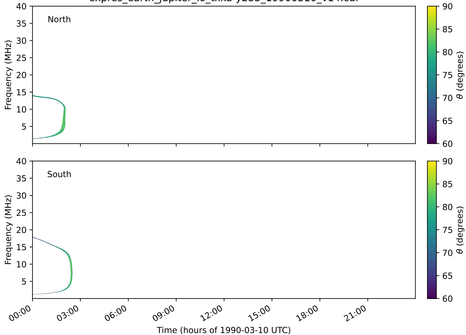
expres_earth_jupiter_io_txka-y235_19900310_v14.cdf
