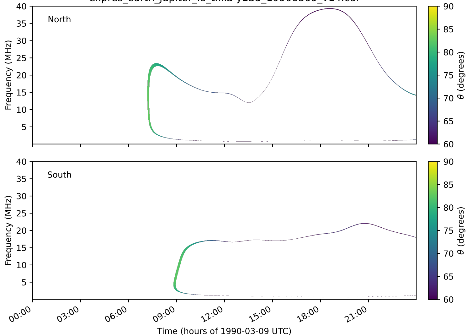
expres_earth_jupiter_io_txka-y235_19900309_v14.cdf
