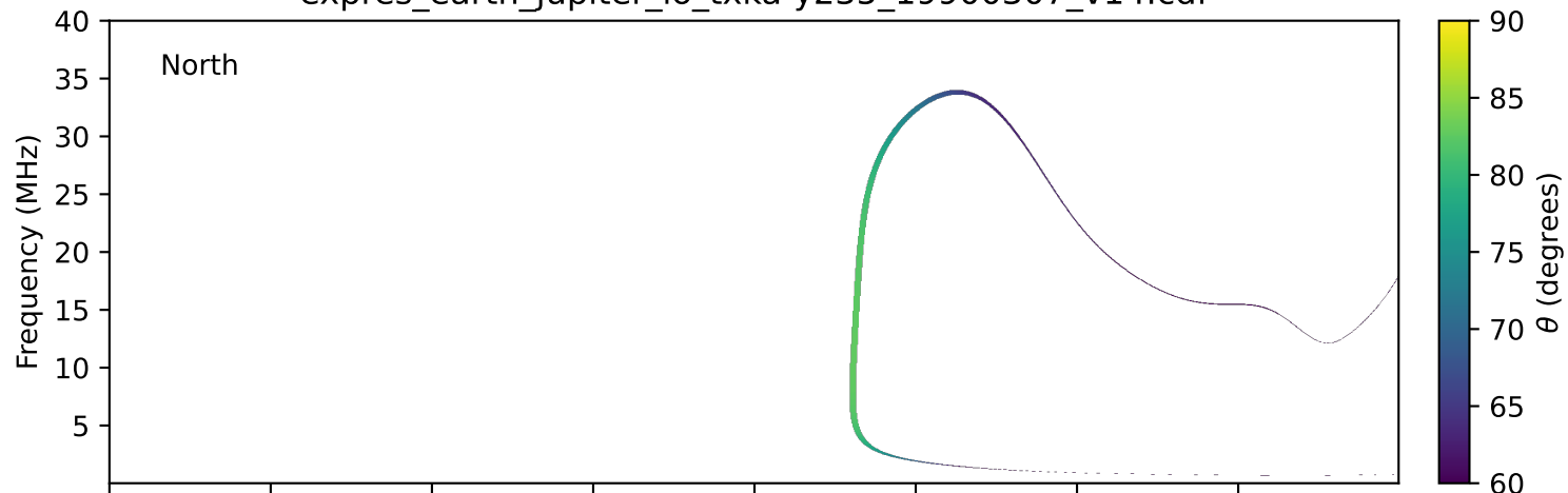
expres_earth_jupiter_io_txka-y235_19900307_v14.cdf
