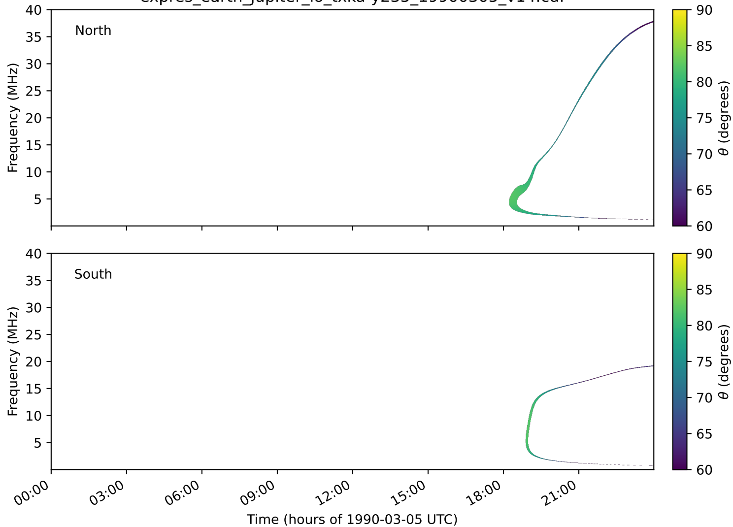
expres_earth_jupiter_io_txka-y235_19900305_v14.cdf
