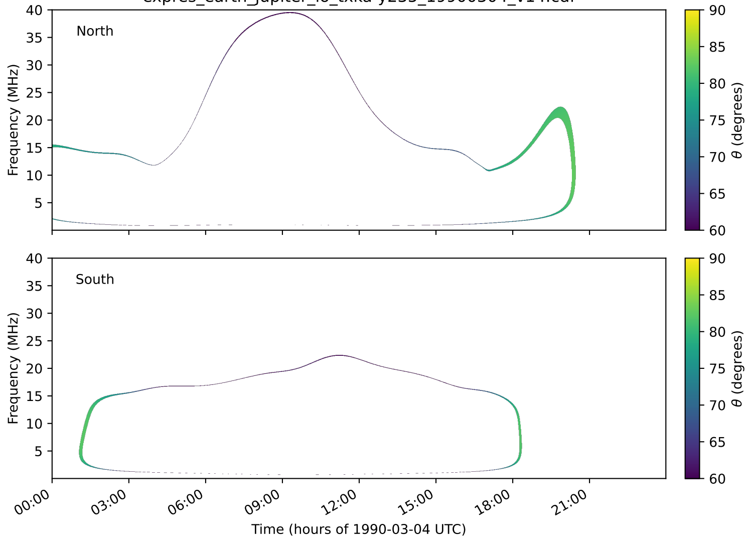
expres_earth_jupiter_io_txka-y235_19900304_v14.cdf
