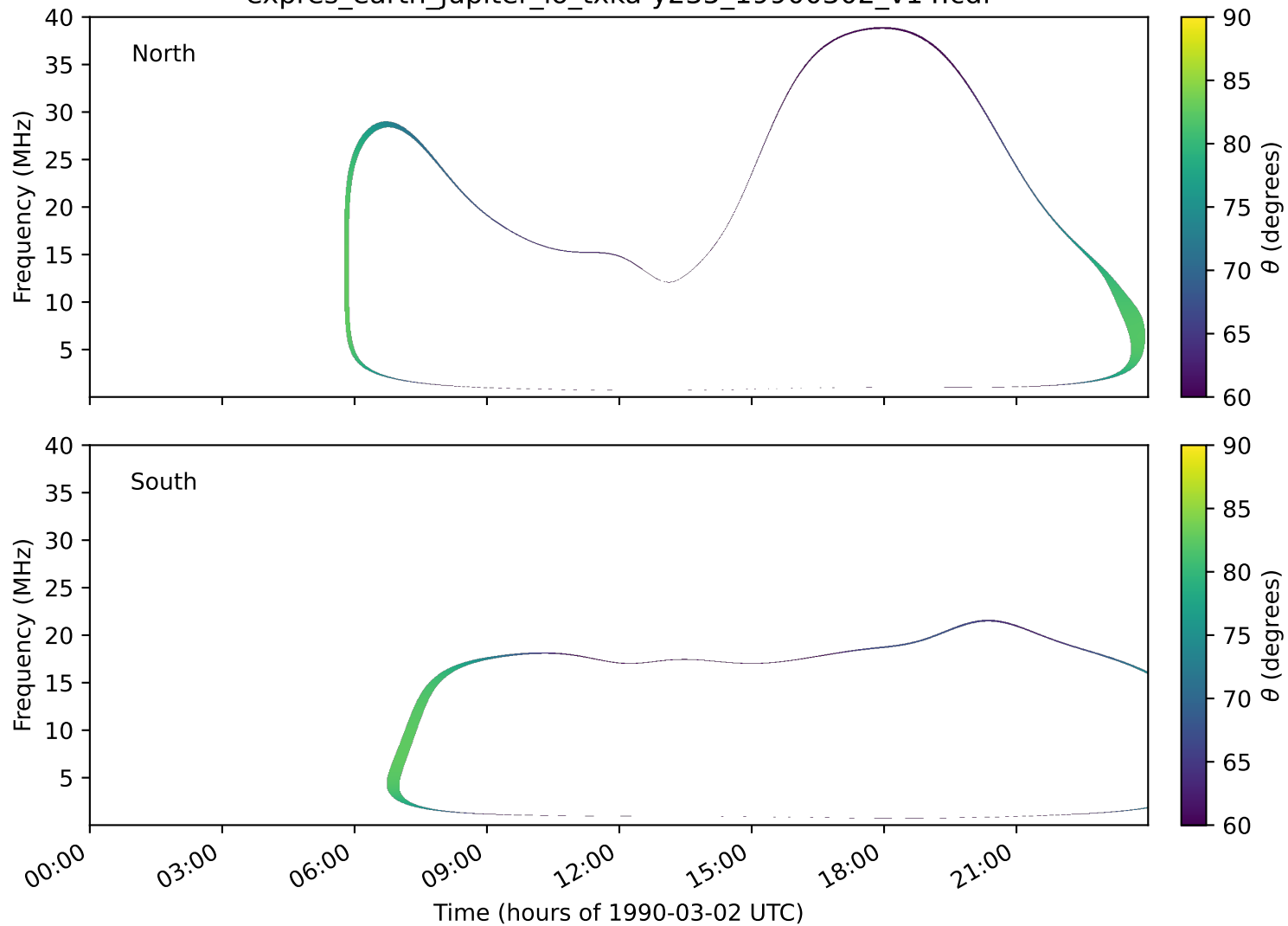
expres_earth_jupiter_io_txka-y235_19900302_v14.cdf
