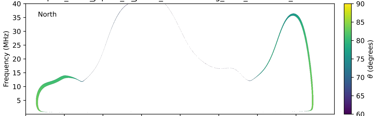
expres_earth_jupiter_io_jrm33_lossc-wid1deg_3kev_19900311_v11.cdf
