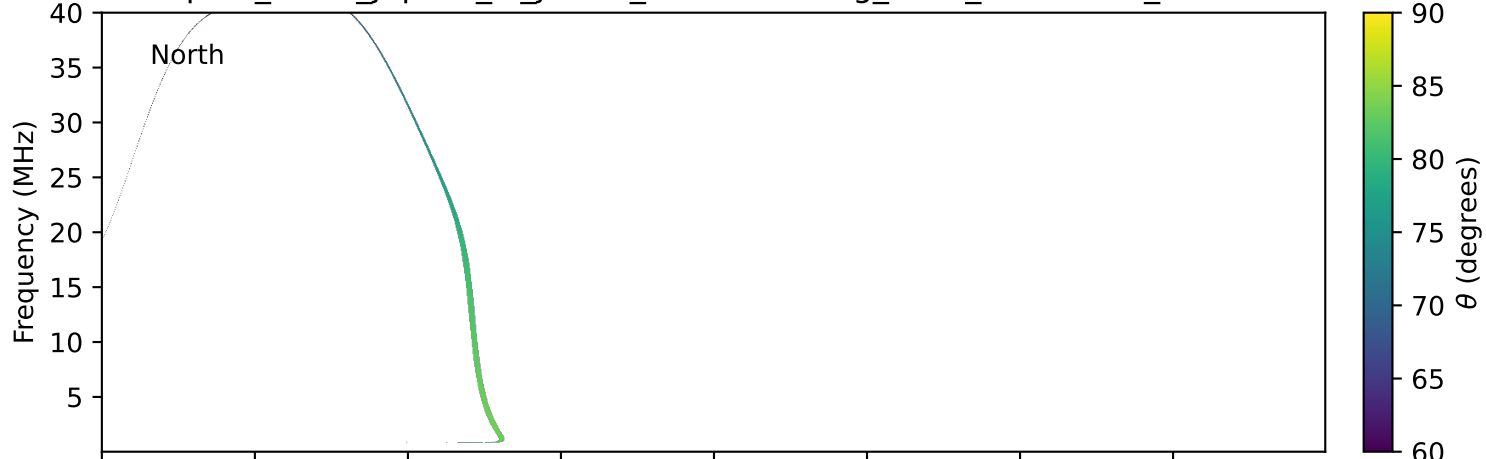
expres_earth_jupiter_io_jrm33_lossc-wid1deg_3kev_19900308_v11.cdf
