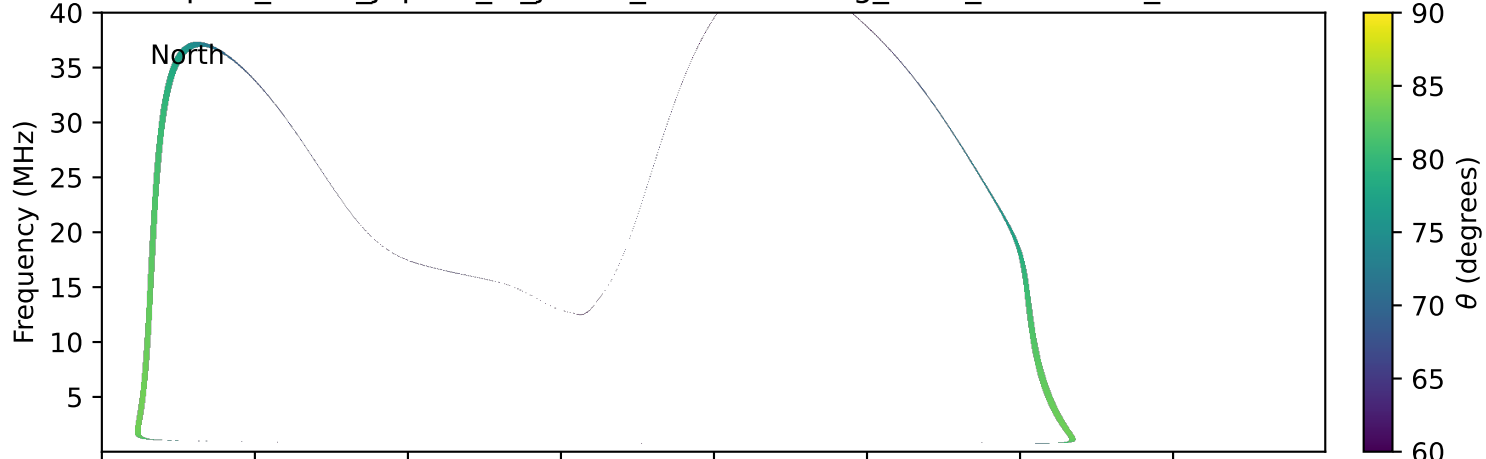
expres_earth_jupiter_io_jrm09_lossc-wid1deg_3kev_19900327_v11.cdf
