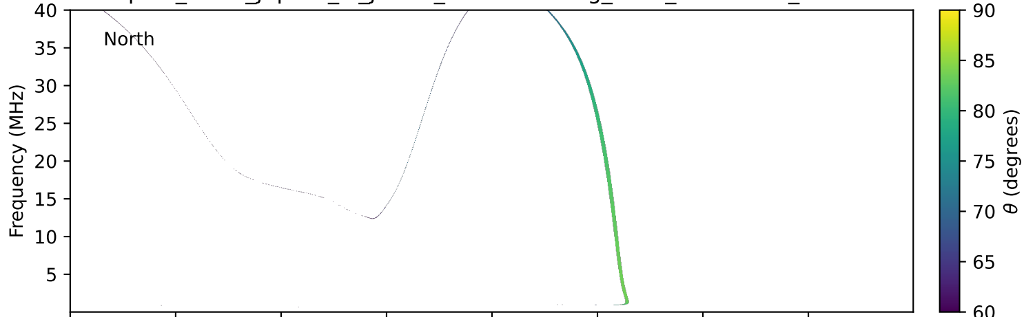
expres_earth_jupiter_io_jrm09_lossc-wid1deg_3kev_19900313_v11.cdf
