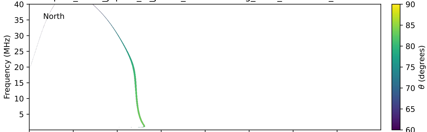
expres_earth_jupiter_io_jrm09_lossc-wid1deg_3kev_19900308_v11.cdf
