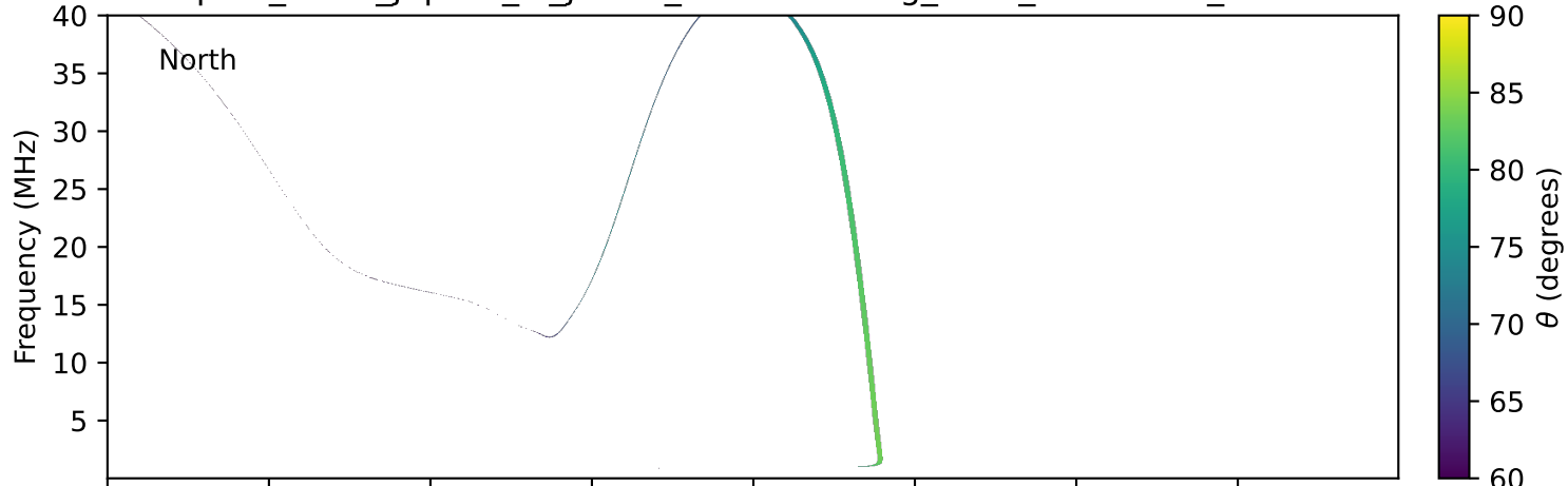
expres_earth_jupiter_io_jrm09_lossc-wid1deg_3kev_19900306_v11.cdf
