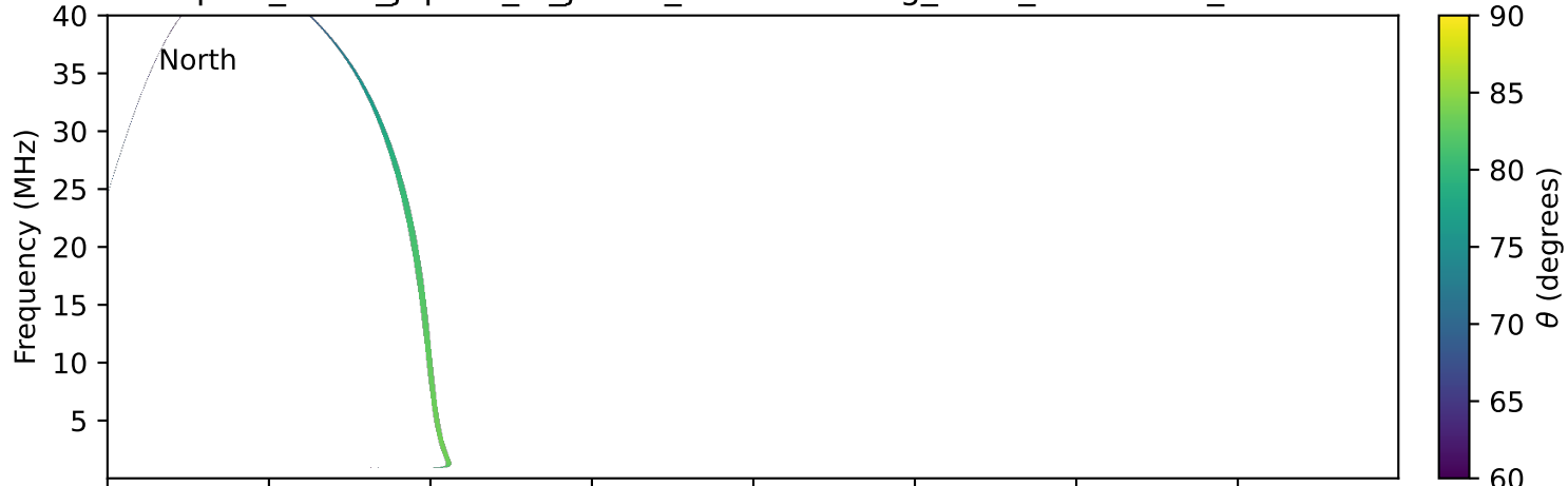
expres_earth_jupiter_io_jrm09_lossc-wid1deg_3kev_19900301_v11.cdf
