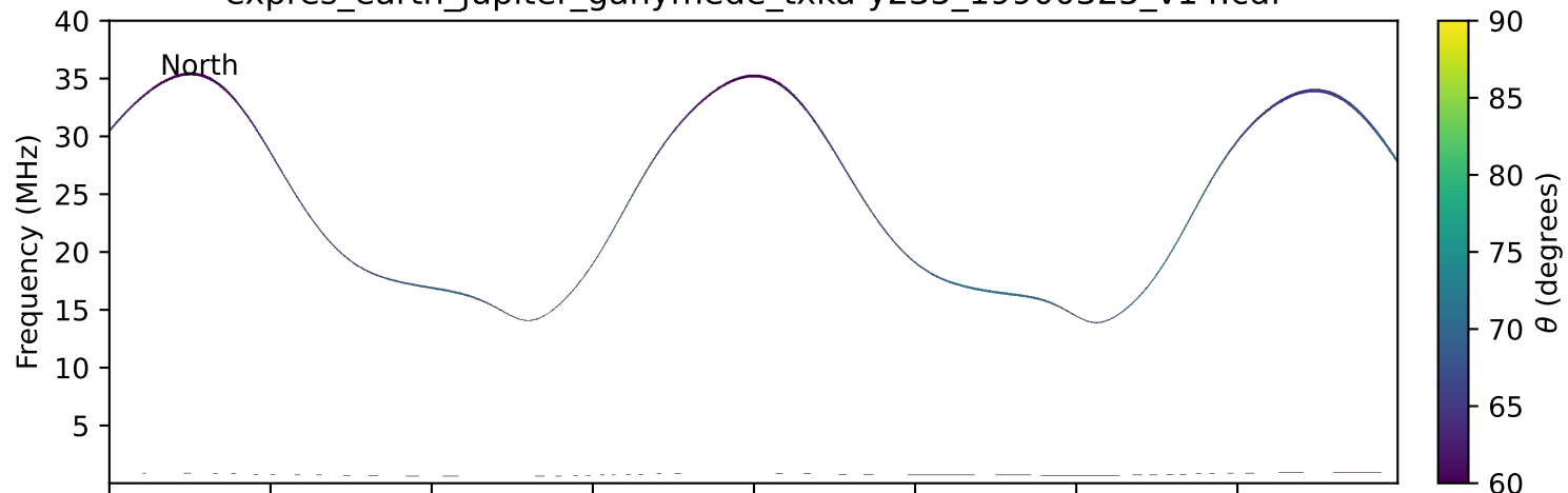
expres_earth_jupiter_ganymede_txka-y235_19900325_v14.cdf
