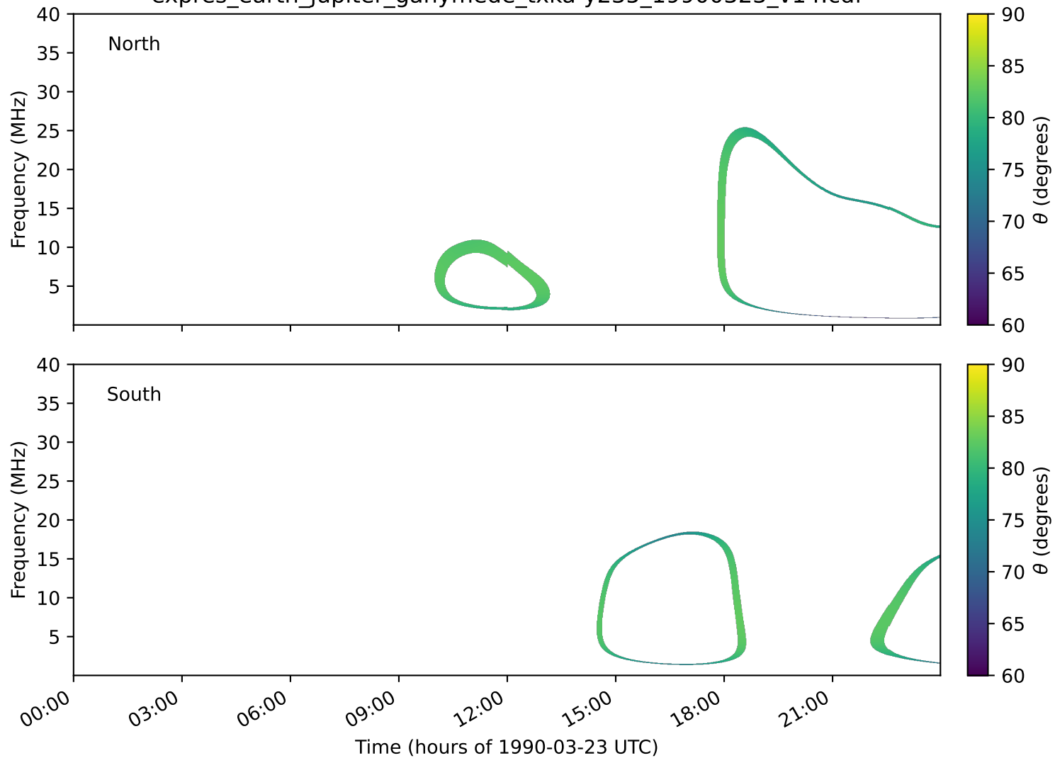
expres_earth_jupiter_ganymede_txka-y235_19900323_v14.cdf
