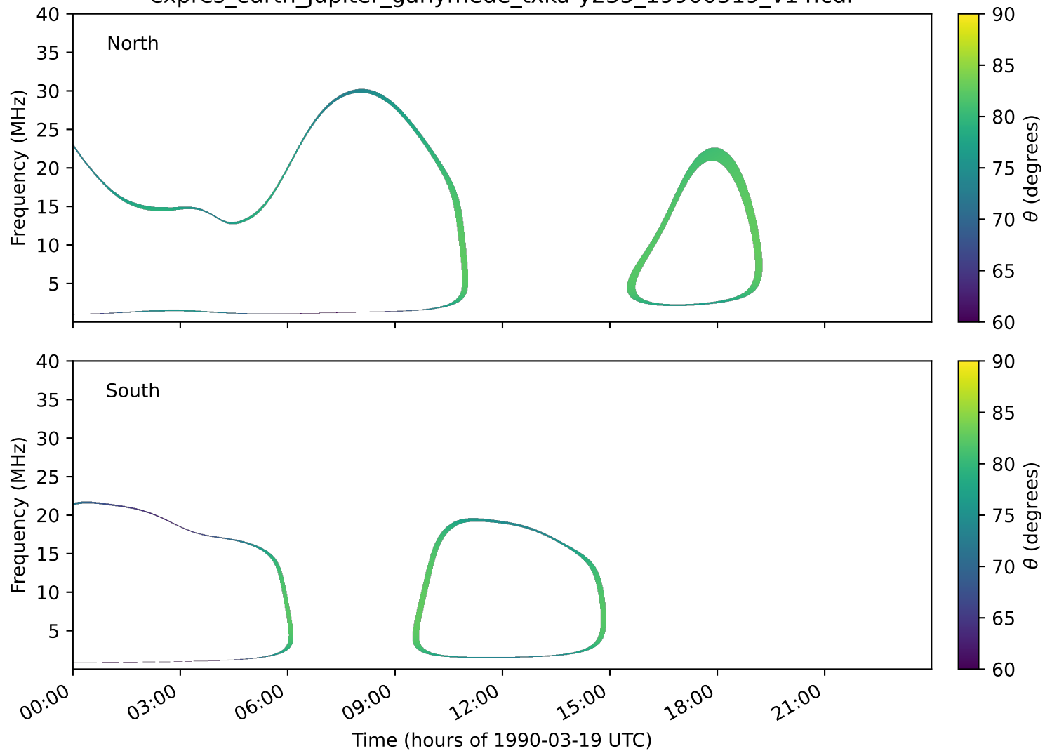
expres_earth_jupiter_ganymede_txka-y235_19900319_v14.cdf
