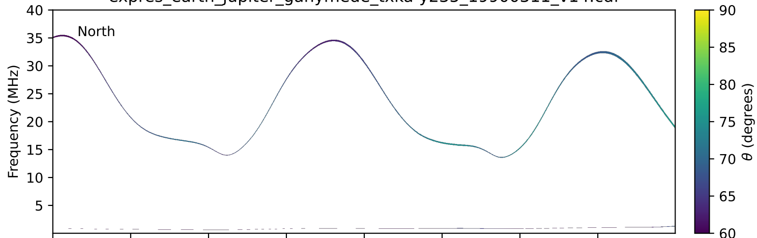
expres_earth_jupiter_ganymede_txka-y235_19900311_v14.cdf
